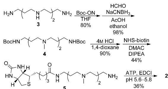
Scheme 1. Synthesis of ATP-polyamine-biotin 2 (APB). Boc-ON = 2-( tert -butoxycarbonyloxyimino)-2-phenylacetoneitrile, DIPEA = diisopropylethylamine, DMAC = dimethylacetamide, EDCl = 1-(3-dimethylaminopropyl)-3-ethylcarbodiimide hydrochloride.
